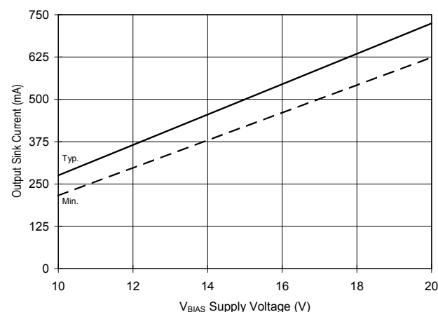
Fig 39b. Output Sink Current Vs. Voltage
