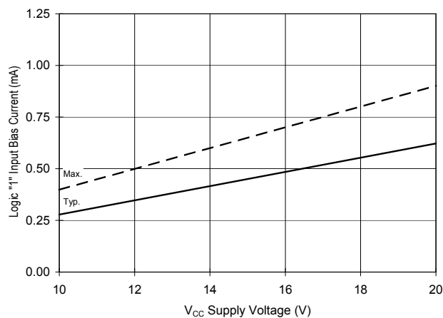
Fig 29b. Logic "1" Input Current Vs. Voltage
