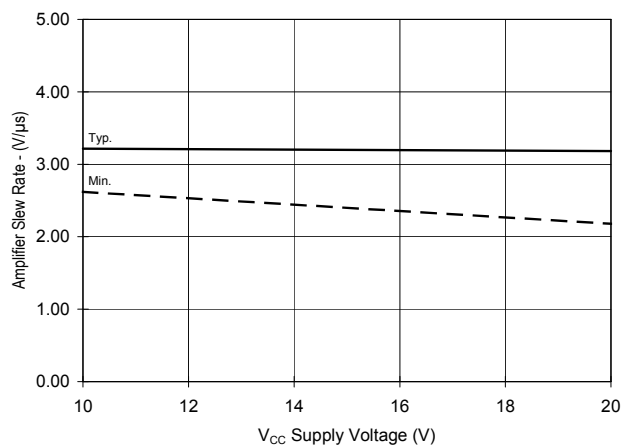
Fig 20b. Amplifier Slew Rate (-) Vs. Voltage
