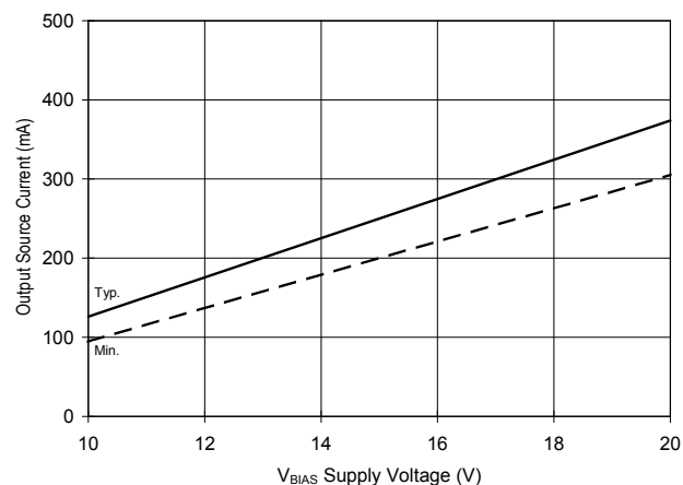
Fig 38b. Output Source Current Vs. Voltage
