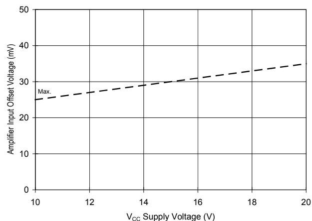
Fig 40b. Amplifier Input Offset Vs. Voltage
