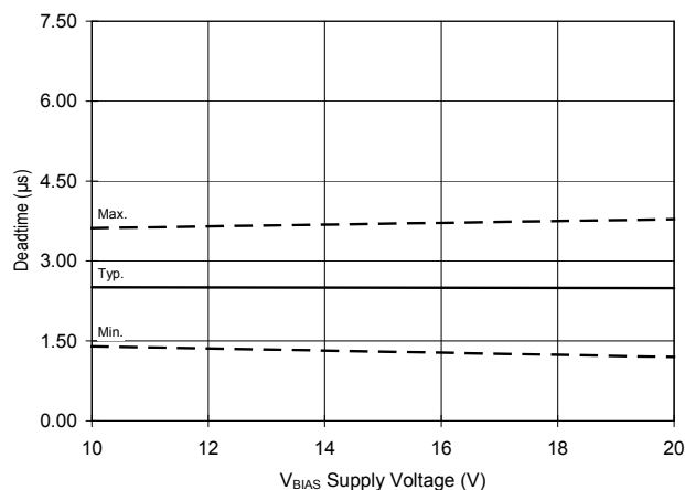
Fig 18b. Deadtime Vs. Voltage
