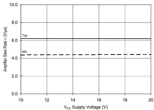
Fig 19b. Amplifier Slew Rate (+) Vs. Voltage
