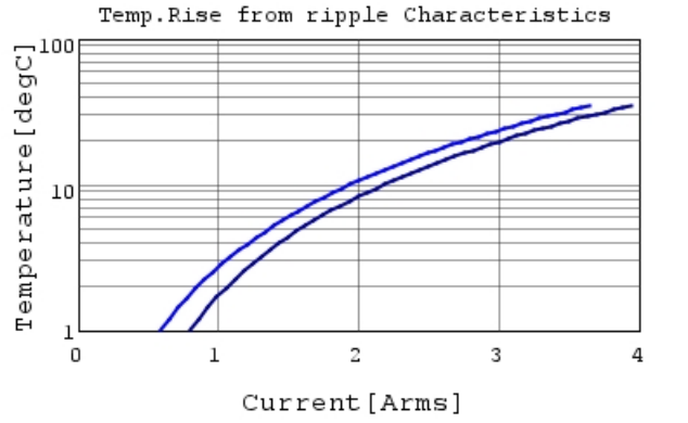
GRM188R61A225KE34 Temp.rise — 500kHz
