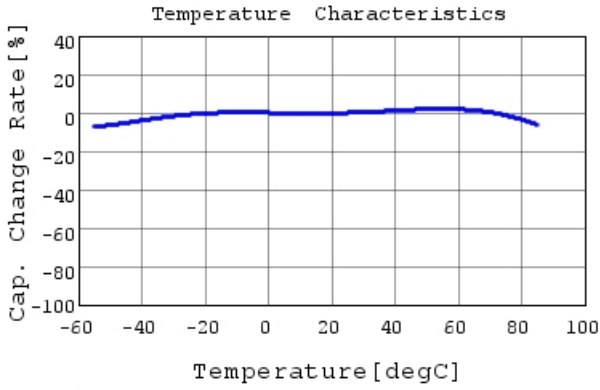
GRM188R61A225KE34 C-Temp. capchange, DC0.0V,
