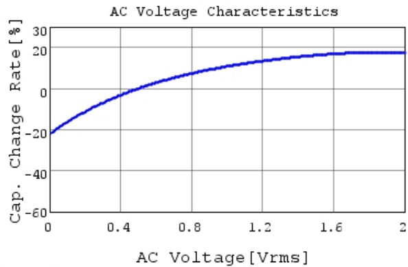
GRM188R61A225KE34 C-AC Voltage capchange, Dc
