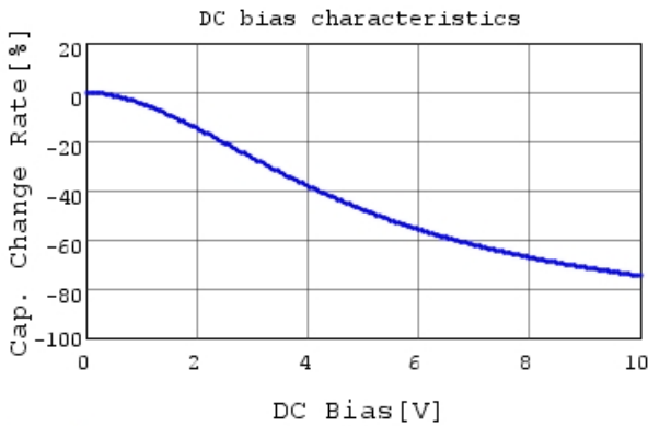
GRM188R61A225KE34 C-DC bias capchange, 25.0c
