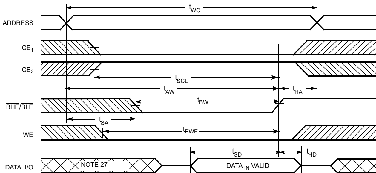
Figure 9. Write Cycle No. 4 ( \overline{BHE/BLER} Controlled, \overline{OE} LOW) [26, 27]
