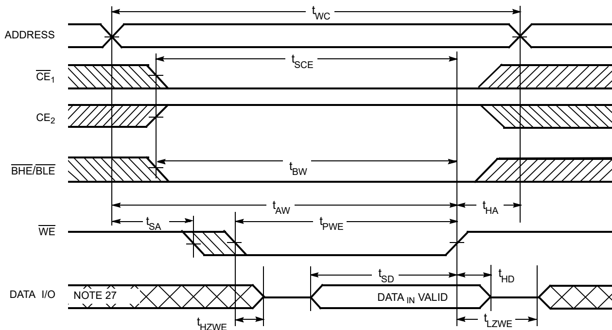
Figure 9. Write Cycle No. 4 ( \overline{BHE/BLER} Controlled, \overline{OE} LOW) [26, 27]
