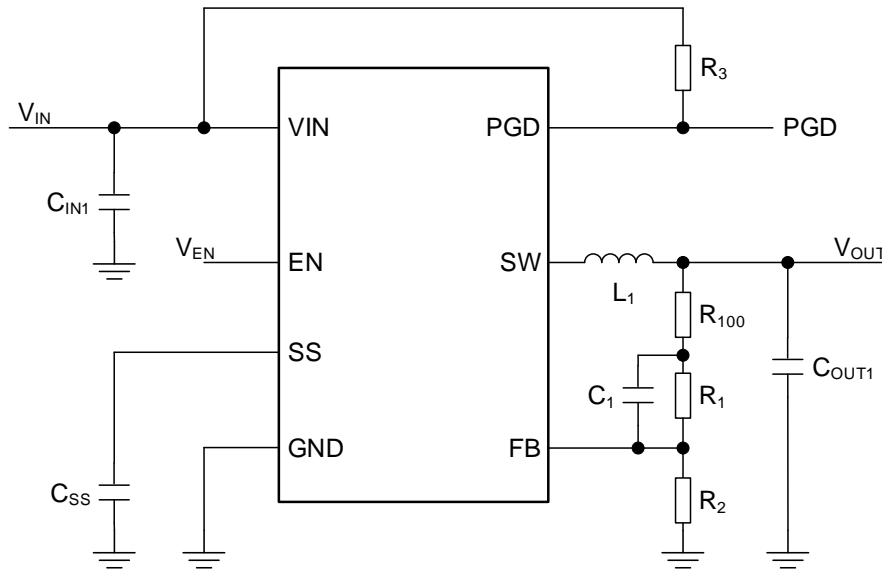
Figure 30. Measurement Circuit 1
