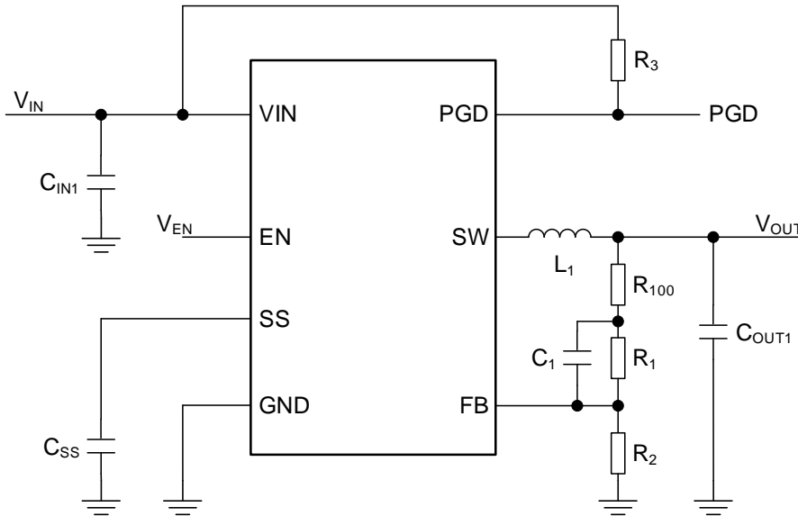
Figure 35. Measurement Circuit 2
