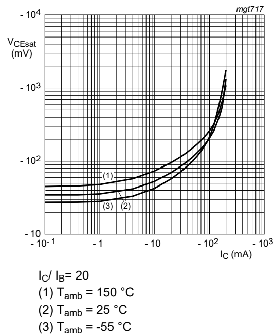
Fig. 10. BC857BQC-Q: Collector-emitter saturation voltage as a function of collector current; typical values
