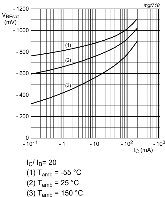
Fig. 11. BC857BQC-Q: Base-emitter saturation voltage as a function of collector current; typical values
