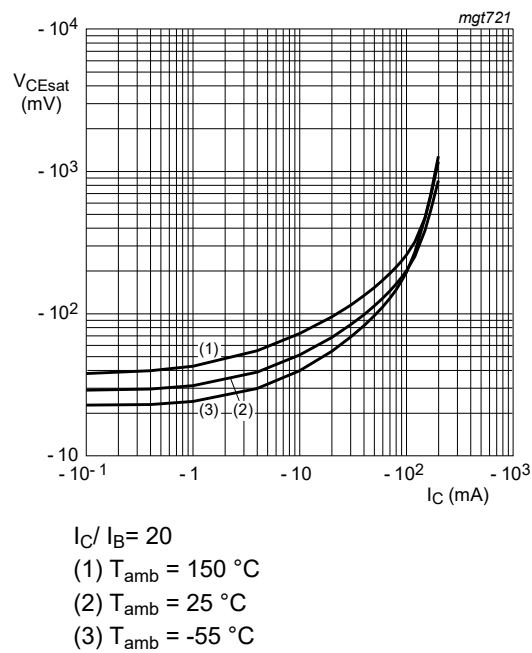
Fig. 14. BC857CQC-Q: Collector-emitter saturation voltage as a function of collector current; typical values
