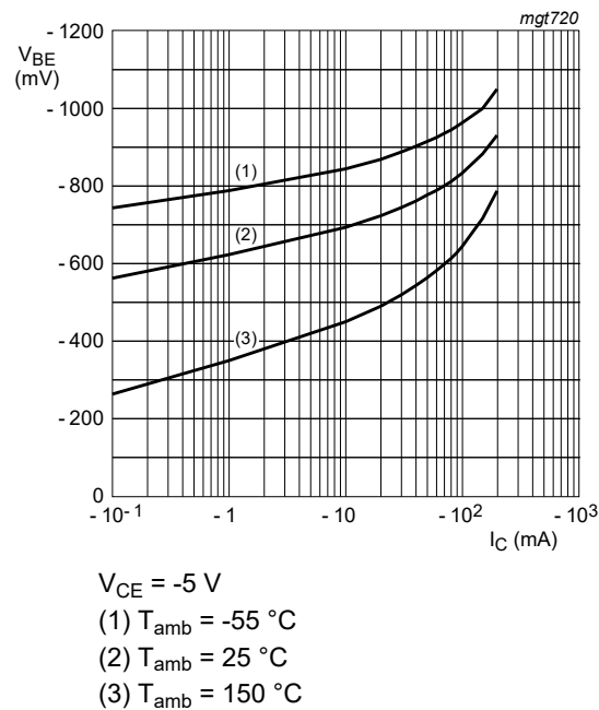
Fig. 13. BC857CQC-Q: Base-emitter voltage as a function of collector current; typical values
