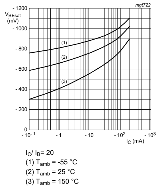
Fig. 15. BC857CQC-Q: Base-emitter saturation voltage as a function of collector current; typical values
