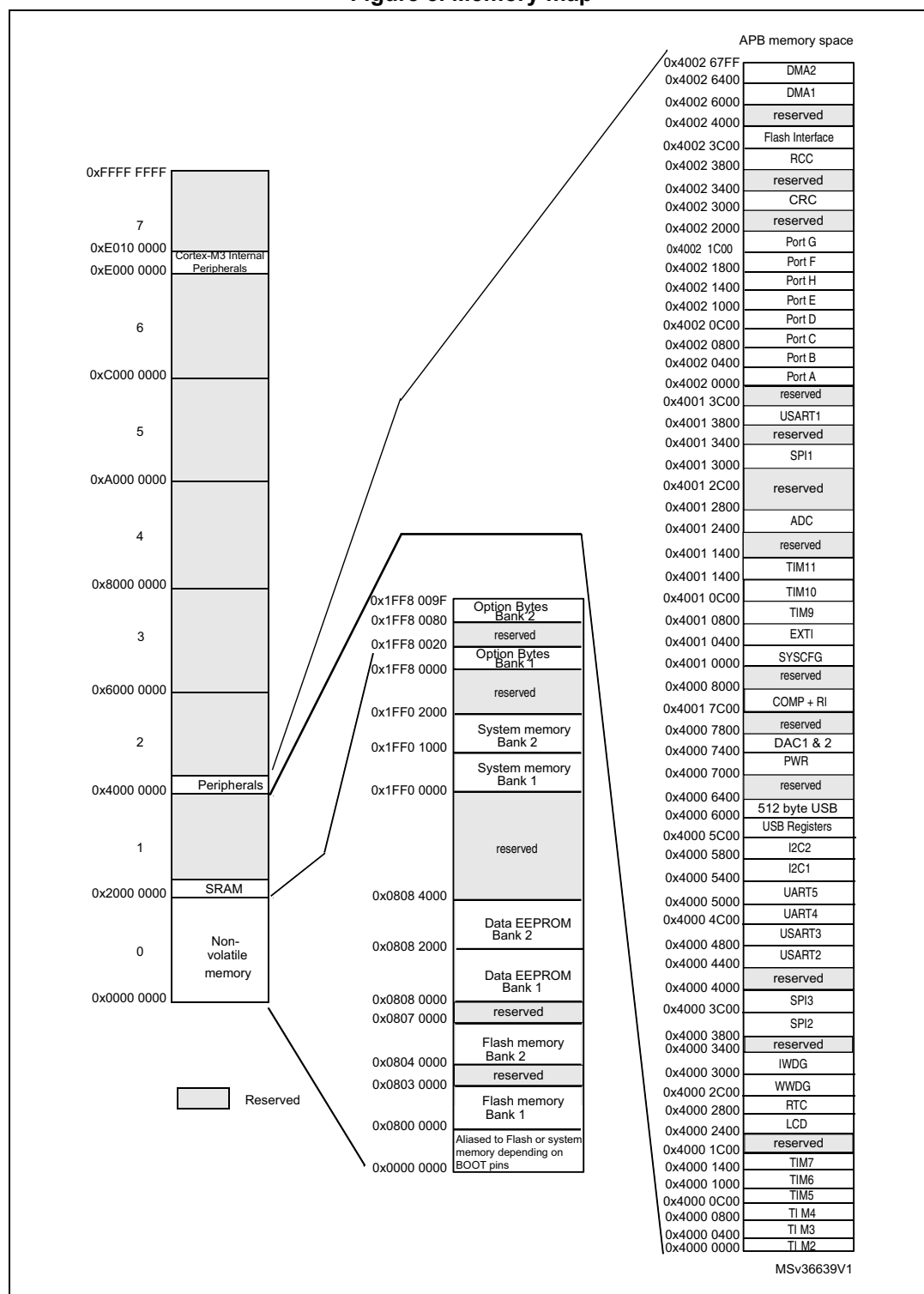
Figure 5. Memory map
