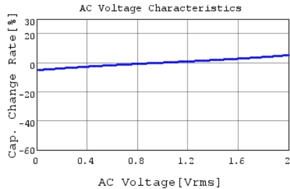
GCJ31CR71H225KA12 C-AC Voltage capchange, DC
