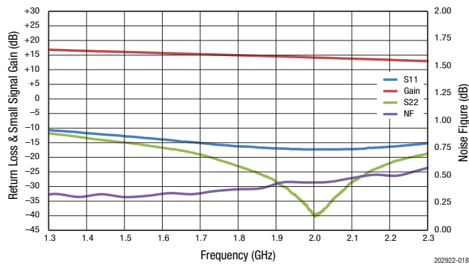
Figure 18. Evaluation Board NF, Gain, and Return Losses for 1400 to 2200 MHz Tuning
