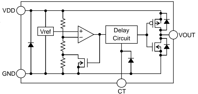
Figure 30. (BD53xx-2M type internal block diagram)
