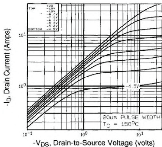
Fig. 2 - Typical Output Characteristics, T_C = 150^\circ C
