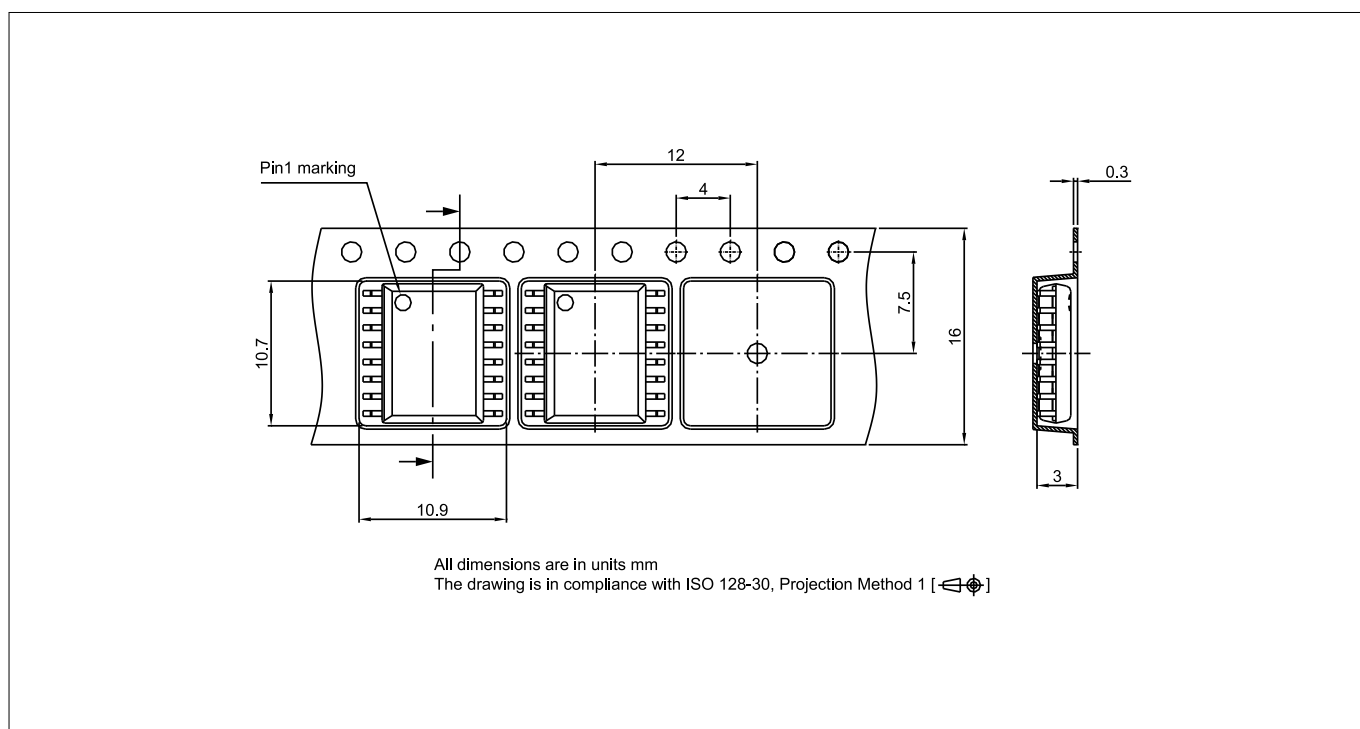
Figure 23 DSO16-300mil packing
