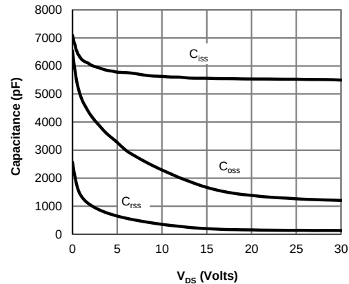
Figure 8: Capacitance Characteristics
