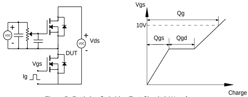
Figure B: Resistive Switching Test Circuit & Waveforms
