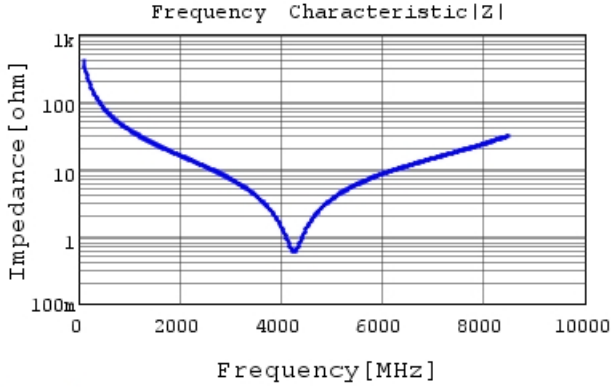
GRM1555C1H4R0CA01 |Z| DCOV, 25degC
