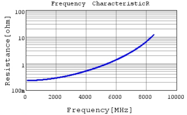
GRM1555C1H4R0CA01 R DCOV, 25degC
