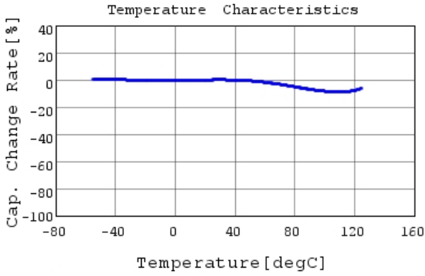
GCM155R72A221KA37 C-Temp. capchange, DC0.0V,
