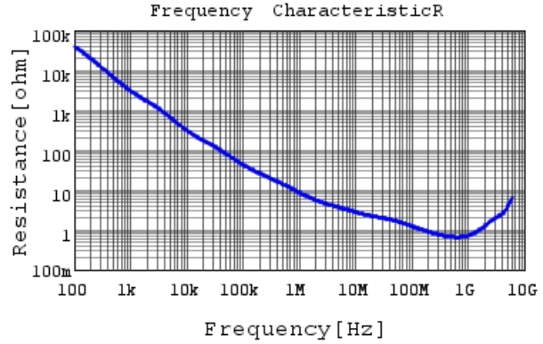
GCM155R72A221KA37 R DC0V, 25degC
