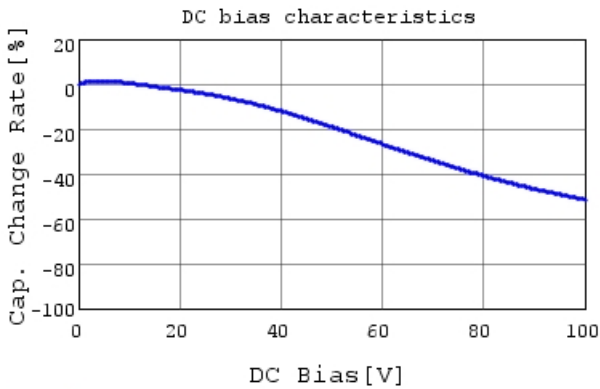
GCM155R72A221KA37 C-DC bias capchange, 25.0c
