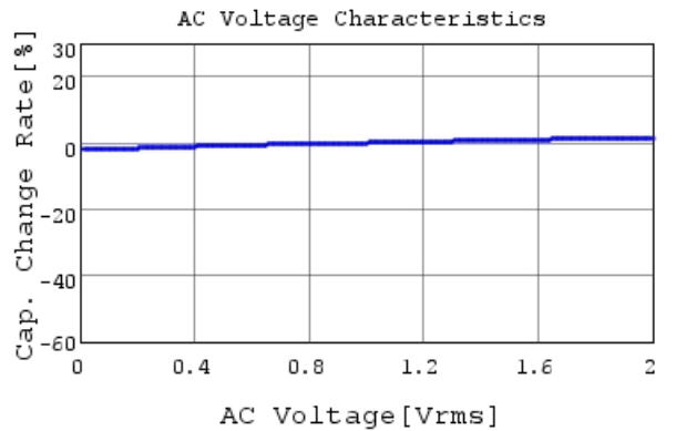
GCM155R72A221KA37 C-AC Voltage capchange, DC
