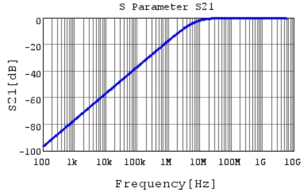
GCM155R72A221KA37 S21 DC0V, 25degC
