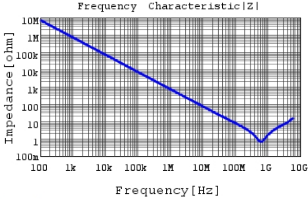
GCM155R72A221KA37 |Z| DC0V, 25degC
