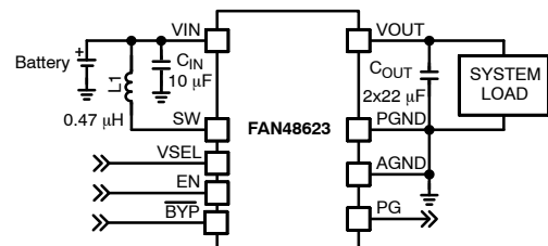
Figure 1. Typical Application
