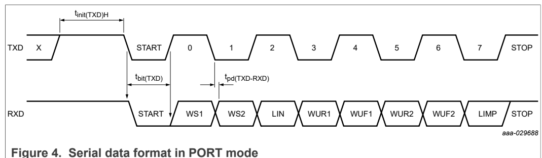
Figure 4. Serial data format in PORT mode
