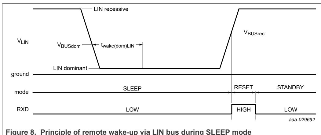
Figure 8. Principle of remote wake-up via LIN bus during SLEEP mode
