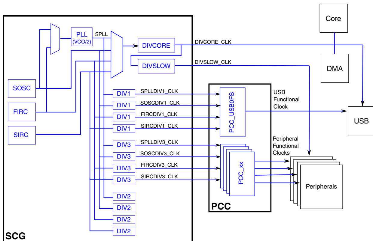
Figure 3. Clock distribution
