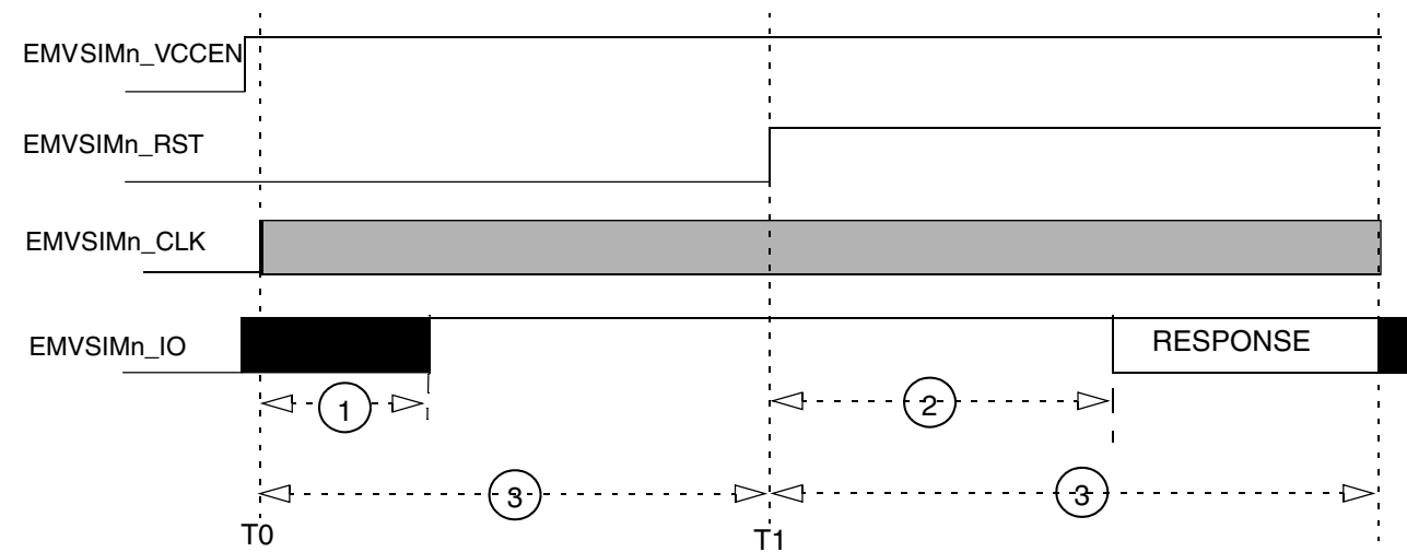
Figure 20. Active-Low-Reset Smart Card Reset Sequence
