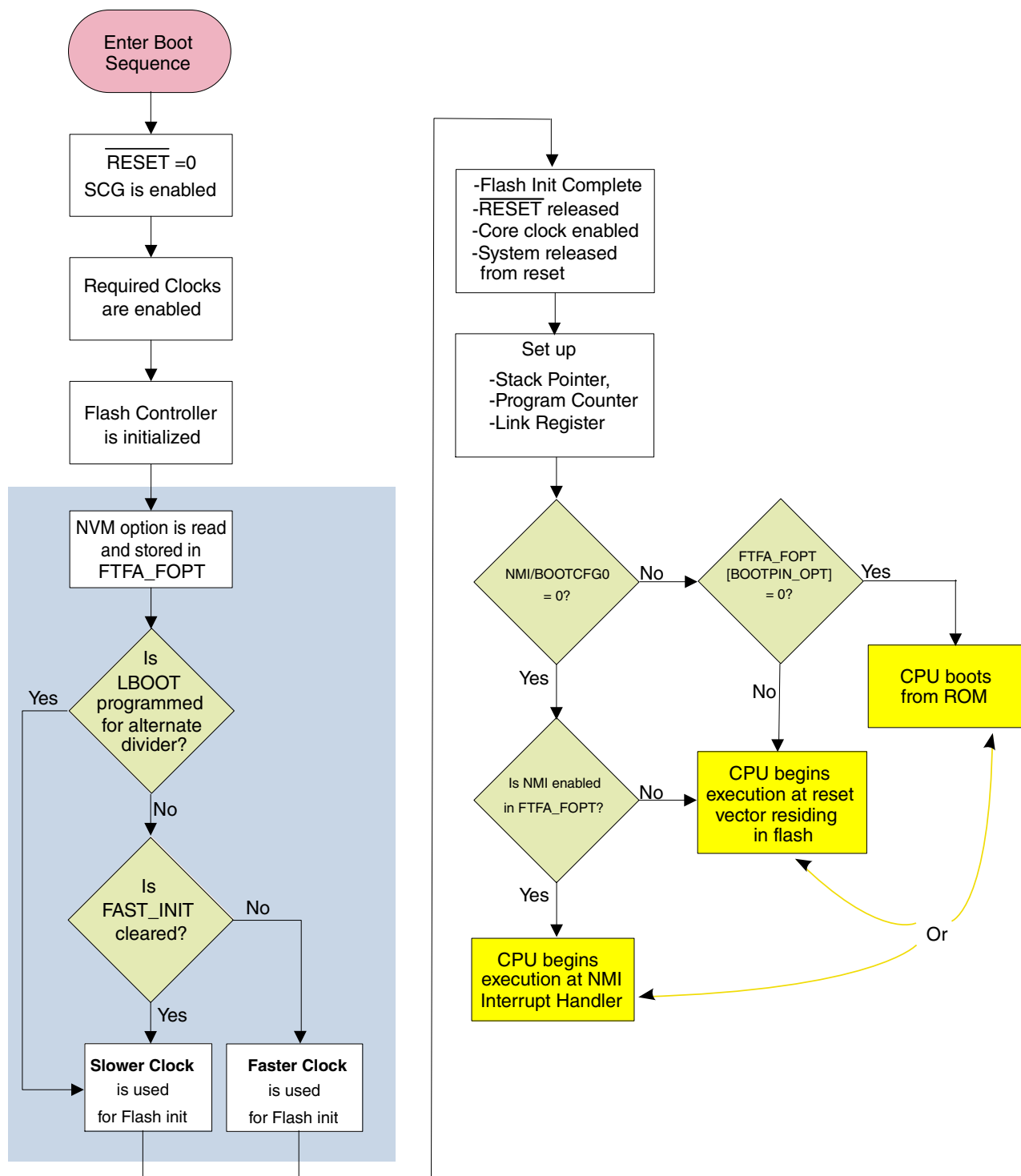
Figure 2. Boot flow chart
