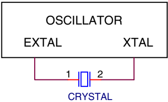
Figure 33. Crystal connection – Diagram 1
