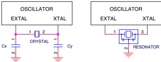
Figure 35. Crystal connection – Diagram 3
