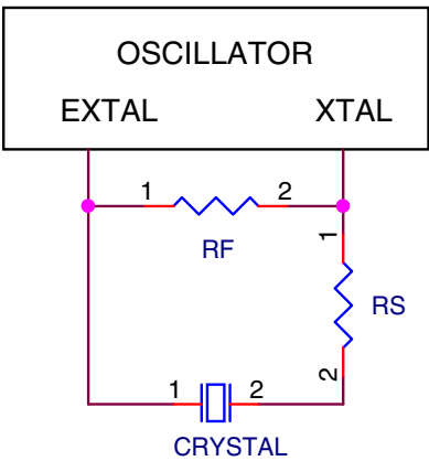
Figure 34. Crystal connection – Diagram 2
