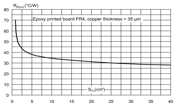
Figure 14: Thermal resistance junction to ambient versus copper surface under tab (D²PAK)
