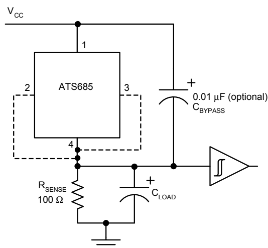
Figure 8. Typical circuit for proper device operation.
