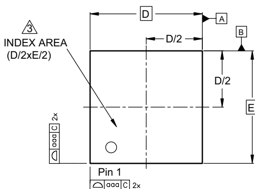
6 TOP VIEW
