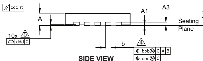
SIDE VIEW
