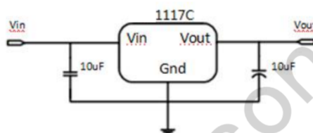
Application circuit of AMS1117 fixed version
