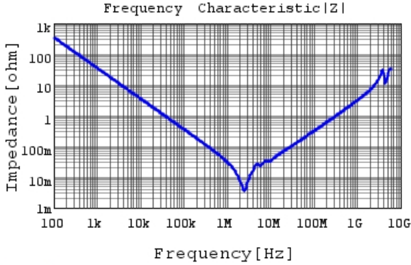
GRM32RR71C475KA01 |Z| DCOV, 25degC
