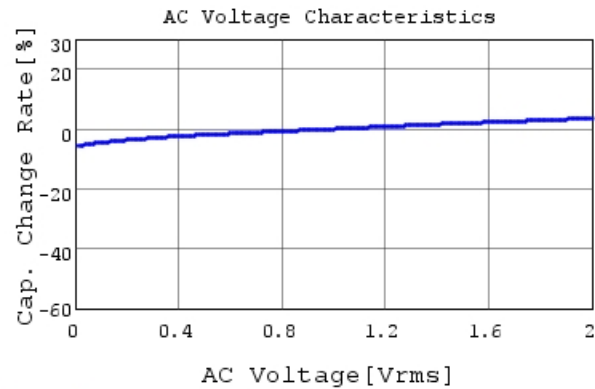
GRM32RR71C475KA01 C-AC Voltage capchange, Dc
