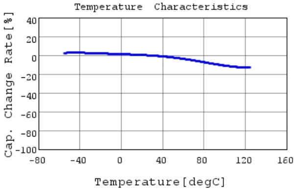
GRM32RR71C475KA01 C-Temp. capchange, DC0.0V,
