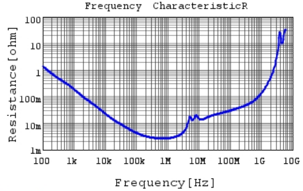
GRM32RR71C475KA01 R DCOV, 25degC
