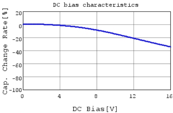
GRM32RR71C475KA01 C-DC bias capchange, 25.0c
