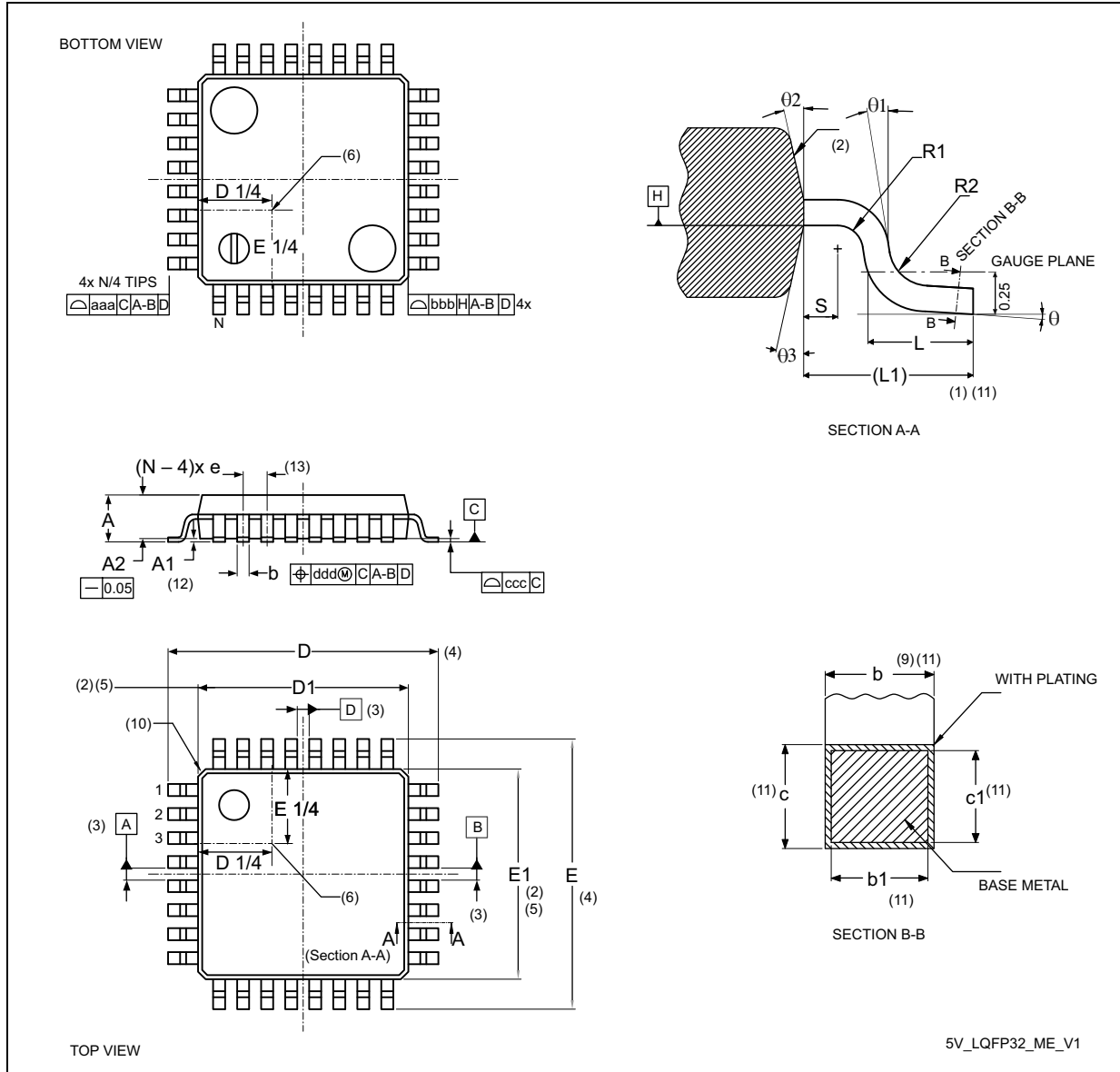
Figure 39. LQFP32 - Outline
