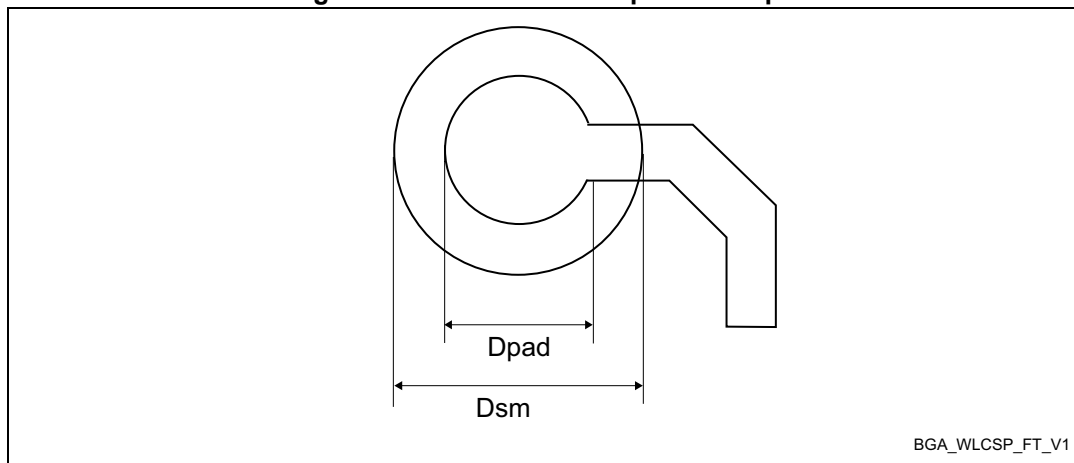
Figure 48. WLCSP52 - Footprint example
