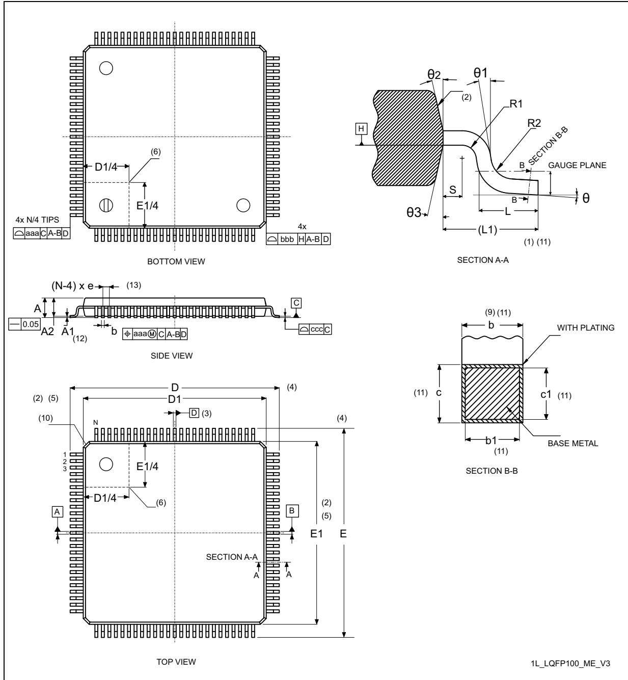
Figure 55. LQFP100 - Outline (15)
