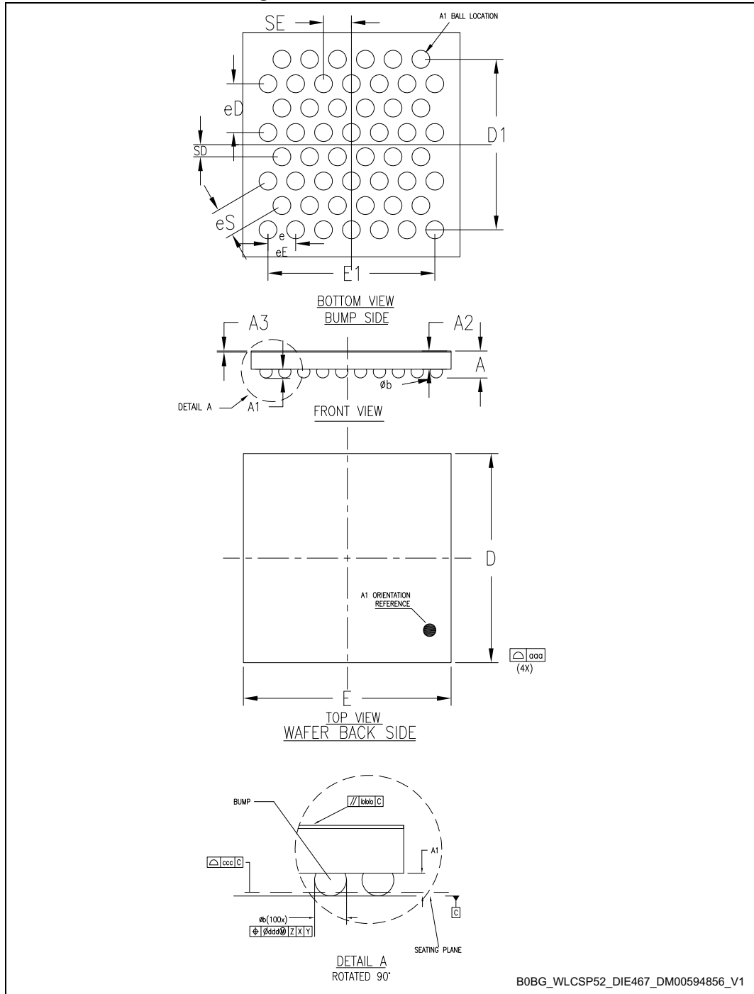
Figure 47. WLCSP52 - Outline
