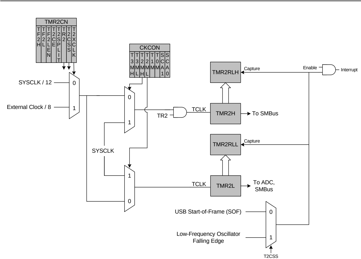
Figure 26.7. Timer 2 Capture Mode (T2SPLIT = 0)
