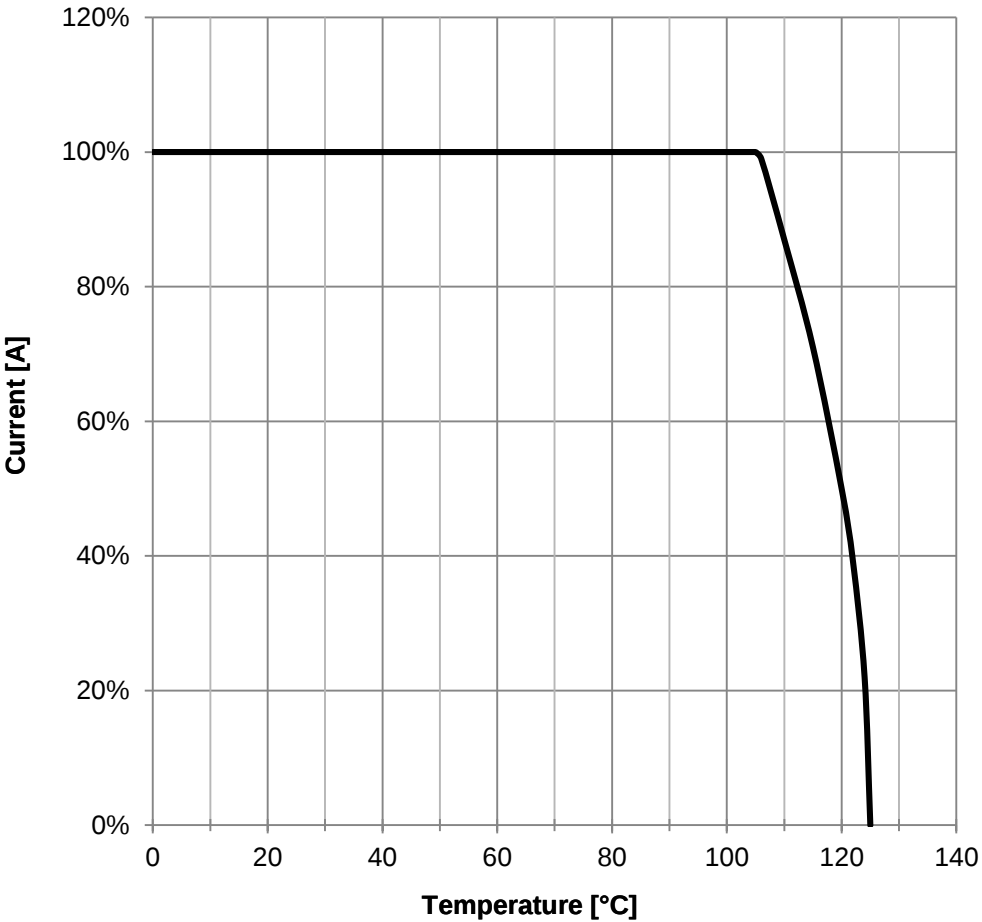
Derating Curve:
