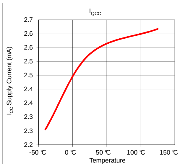
Figure 9: Icc Quiescent Current vs. Temperature
