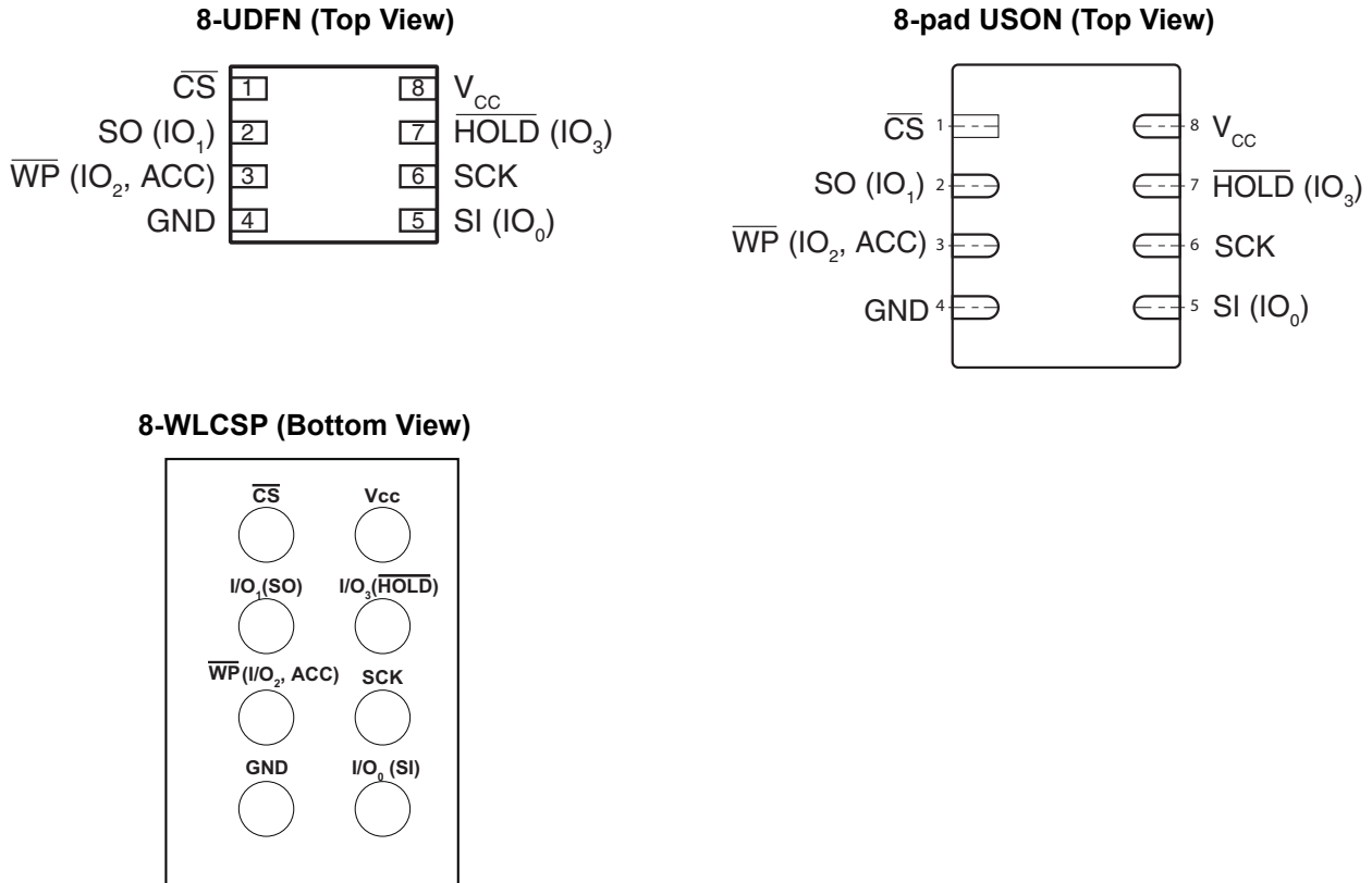
Figure 1. Package Types
