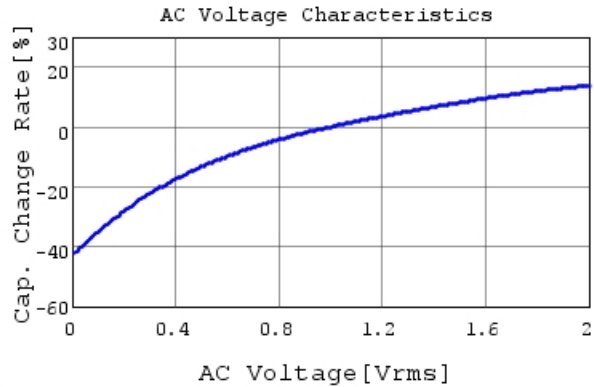
GRM21BR71A475KA73 C-AC Voltage capchange, Dc
