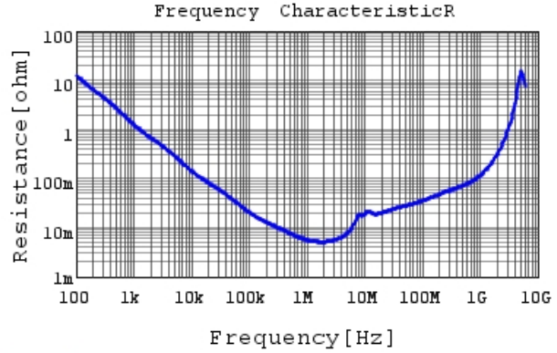
GRM21BR71A475KA73 R DCOV, 25degC
