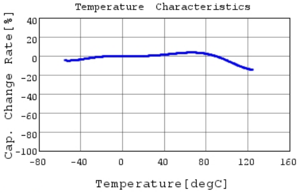
GRM21BR71A475KA73 C-Temp. capchange, DC0.0V,
