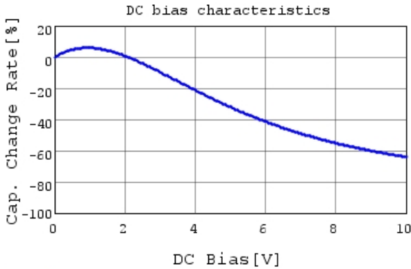
GRM21BR71A475KA73 C-DC bias capchange, 25.0c
