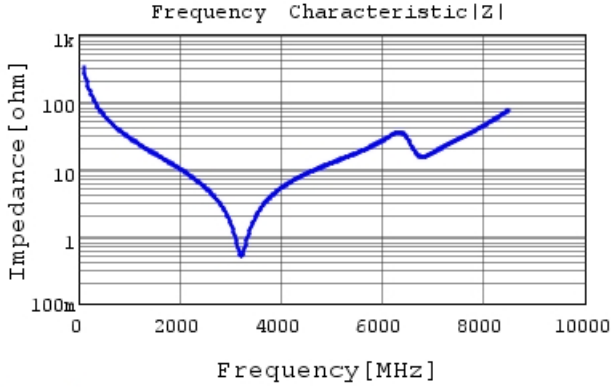
GRM1885C1H5R0CA01 |Z| DCOV, 25degC
