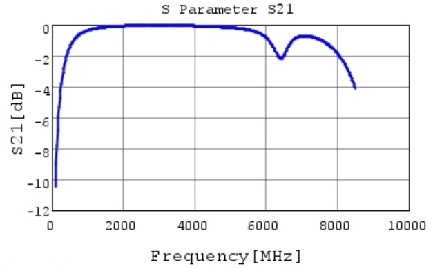
GRM1885C1H5R0CA01 S21 DCOV, 25degC
